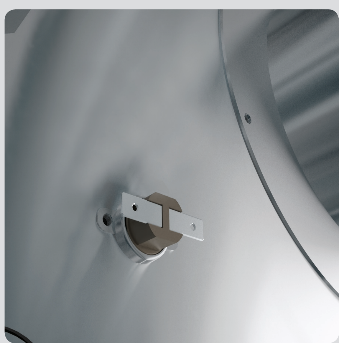
A. Safety thermostat and T2 probe placed at the exhaust
